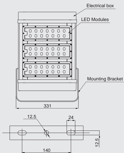
Mounting Holes
