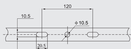
Mounting hole drawing
