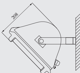
Side wall-mounting
